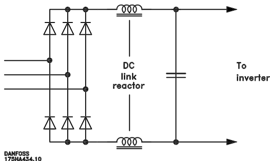
DC link reactors as standard.
