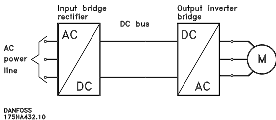
Figure 1: General block diagram of a variable frequency drive.
