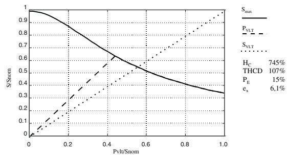
Figure 8: Distribution of linear load and drive load
