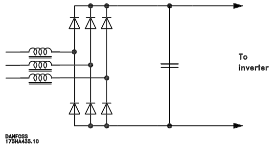
Figure 15: With a conventional variable frequency drive, AC line reactors have to be added in HVAC installations.
