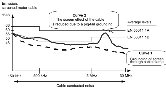
Figure 5: Comparison between good installation and pigtail installation
