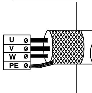
Figure 3: Motor cable with pigtail
