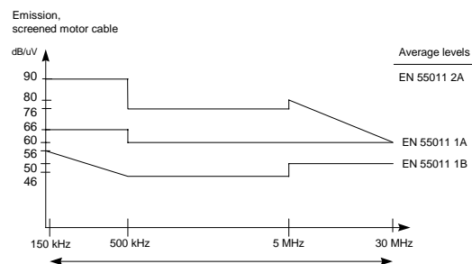
Figure 2: Average conducted emission levels
