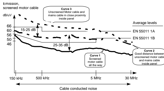
Figure 6: Using unscreened cables inside the panel.
