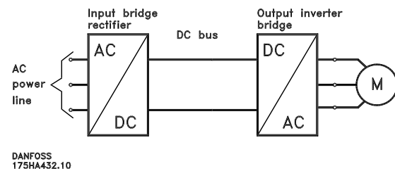
Figure 1: Schematic of Basic Drive design
