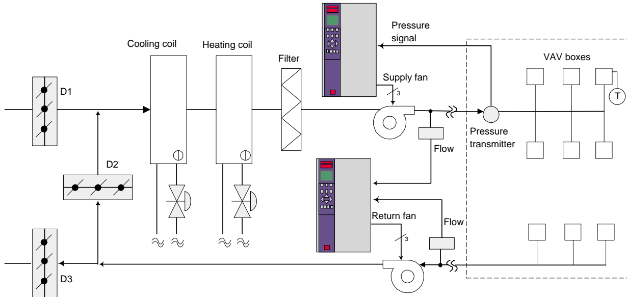
Fig. 2 The VLT frequency converter solution
