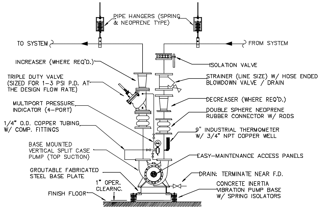
4 VERTICAL SPLIT CASE (TOP SUCTION) PUMP DETAIL — (BASE MOUNTED ON A CONCRETE INERTIA PAD) NOT TO SCALE
